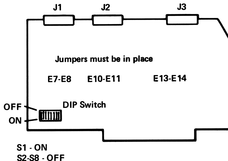
Figure 2. DIP Switch Settings
